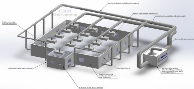
1) 3D HVAC Design (3D Layout Plan)
